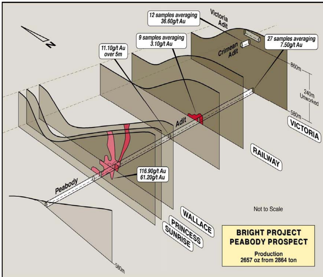
Figure 3: BRIGHT GOLD PROJECT - PEABODY GOLD PROSPECT & ASSOCIATED REEF LINES ISOMETRIC DIAGRAM Extracts from Dynasty's 2005 Prospectus
